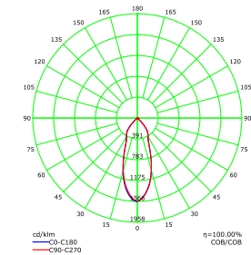
Luminous Intensity Distribution Curve(cd/klm)
